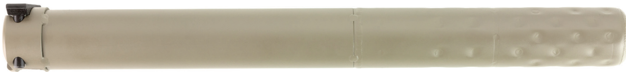
M110 SUPPRESSOR 7.62/.300 PN: 24611 Connects to SR-25 gas block. For rifles with M110 flash hider only. Gate Latch Connector Length: 14" Weight: 32.0 oz NSN: 1005-01-542-4487
