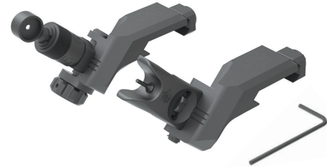
45° OFFSET CLAMP MOUNT FOLDING SIGHT KIT P/N: 31593
